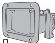
□ Latches, Rotary Paddle Handle, Left. Part Number 454.42 - Qty - 1 Right. Part Number 454.43 - Qty - 1
