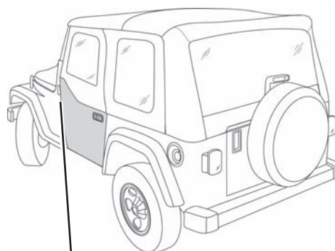
□ Latches, Rotary Paddle Handle, Left. Part Number 454.42 - Qty - 1 Right. Part Number 454.43 - Qty - 1
